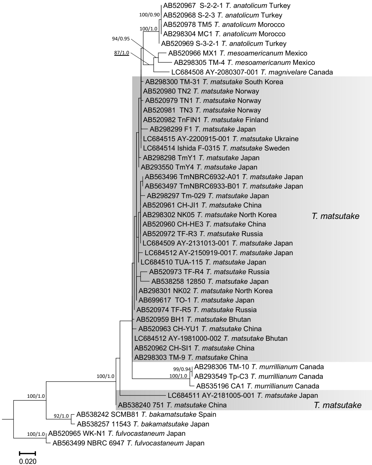
Supplementary Fig. S3 – ML phylogenetic tree of the megB1 of Tricholoma matsutake and closely related species in the section Caligata . Bootstrap (BS) values > 60% from ML trees (left) and Bayesian posterior probabilities (PP) > 0.60 (right) are shown near the nodes. Thick nodes indicate significant support by both the BS (> 85%) and PP (> 1.0) values. Taxon names in bold indicate the specimens examined in this study.
