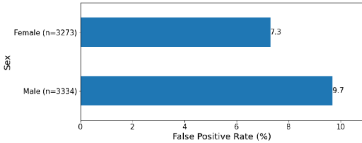
Supplementary Figure 6: False Positive Rates by sex in the testing cohort (DermIS and PAD-uefs 20).
