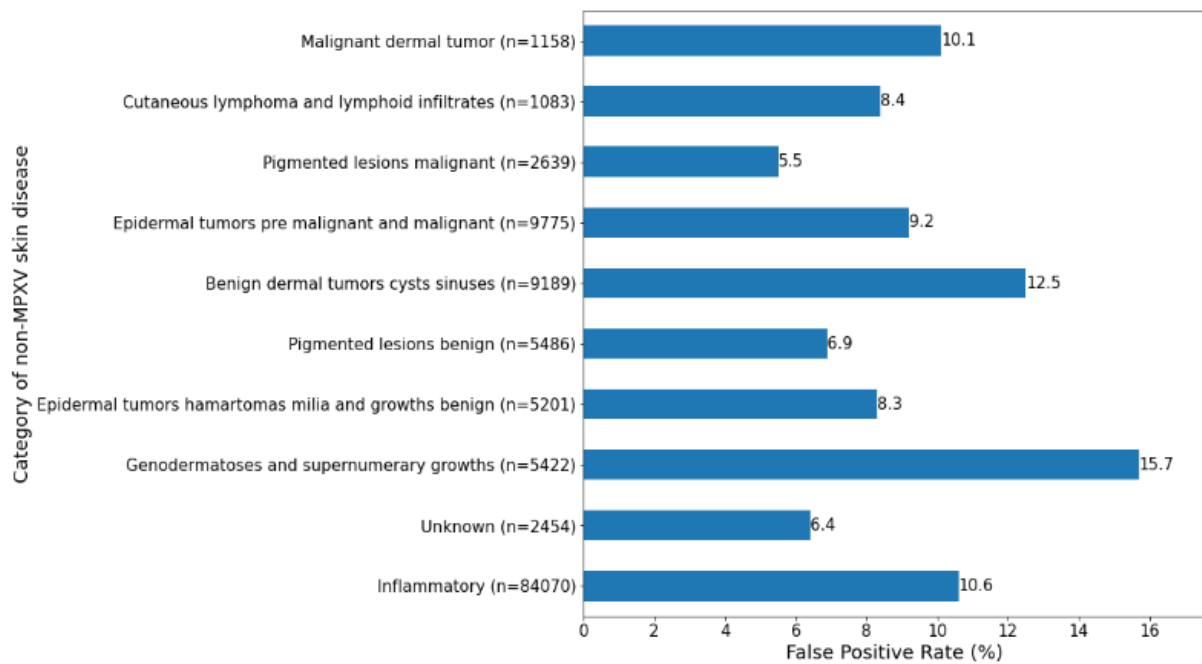
Supplementary Figure 2: False Positive Rates by category of non-MPXV skin disease in the testing cohort.
