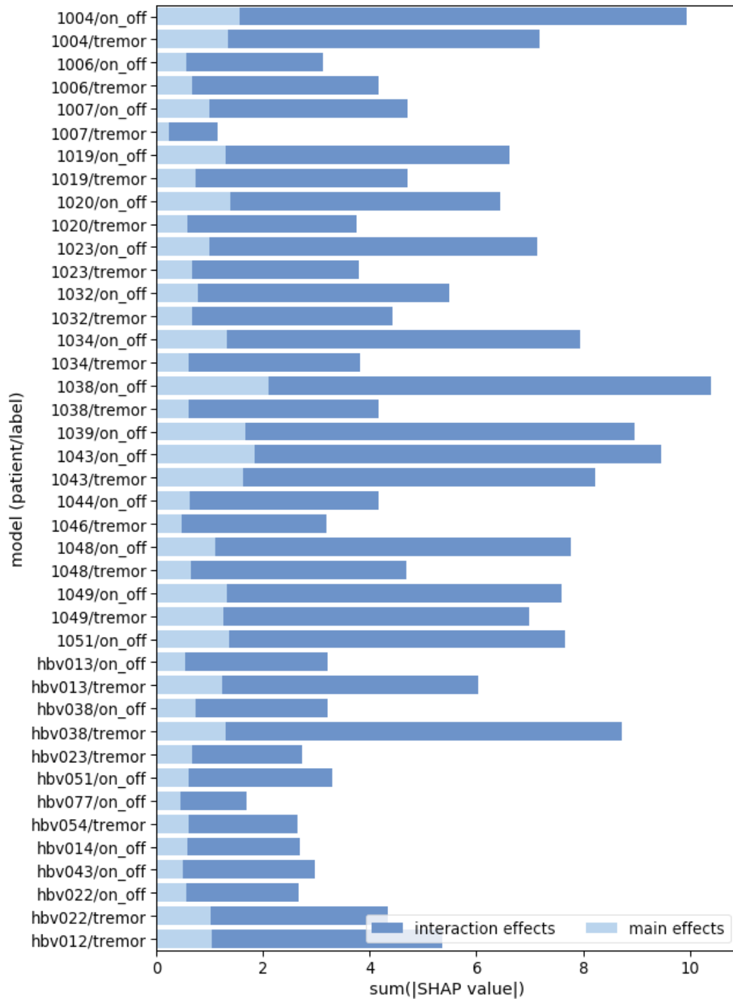
S2 Fig: Sum of magnitudes of SHAP interaction values with main and interaction effects separately, shown for the winning models of team dbmi in SC1 and SC3. Interaction effects outweigh main effects in all models
