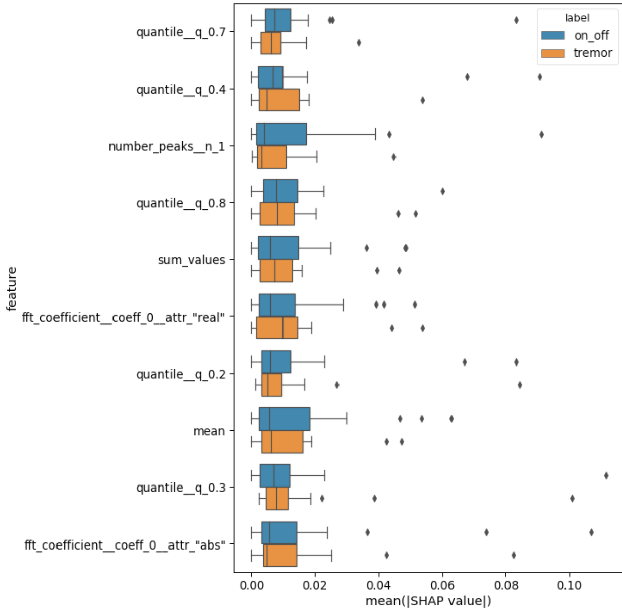
S3 Fig: Distributions of SHAP magnitude for the top 10 features over models for tremor (SC3) and on_off (SC1) labels for the winning models of team dbmi. quantile__q_{0.2, 0.3, 0.4, 0.7, 0.8} are the 20, 30, 40, 70, and 80th data percentiles, respectively; number_peaks_n_1 is defined as the number of peaks of at least support 1; sum_values is the sum over time series values; mean is the mean time series value; and fft_coefficient_coeff_0_attr_{"real", "abs"} are the real component and absolute value of the 0th coefficient of the fast Fourier Transform (0 Hz), respectively.
