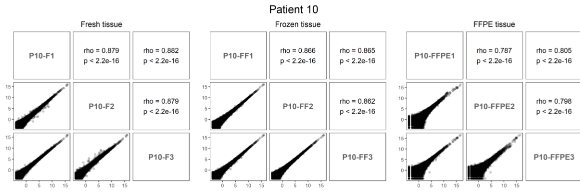
S2 Fig: Spearman's correlation analysis of replicate RNA sequencing investigations in fresh, frozen, and FFPE tissues - continued.
