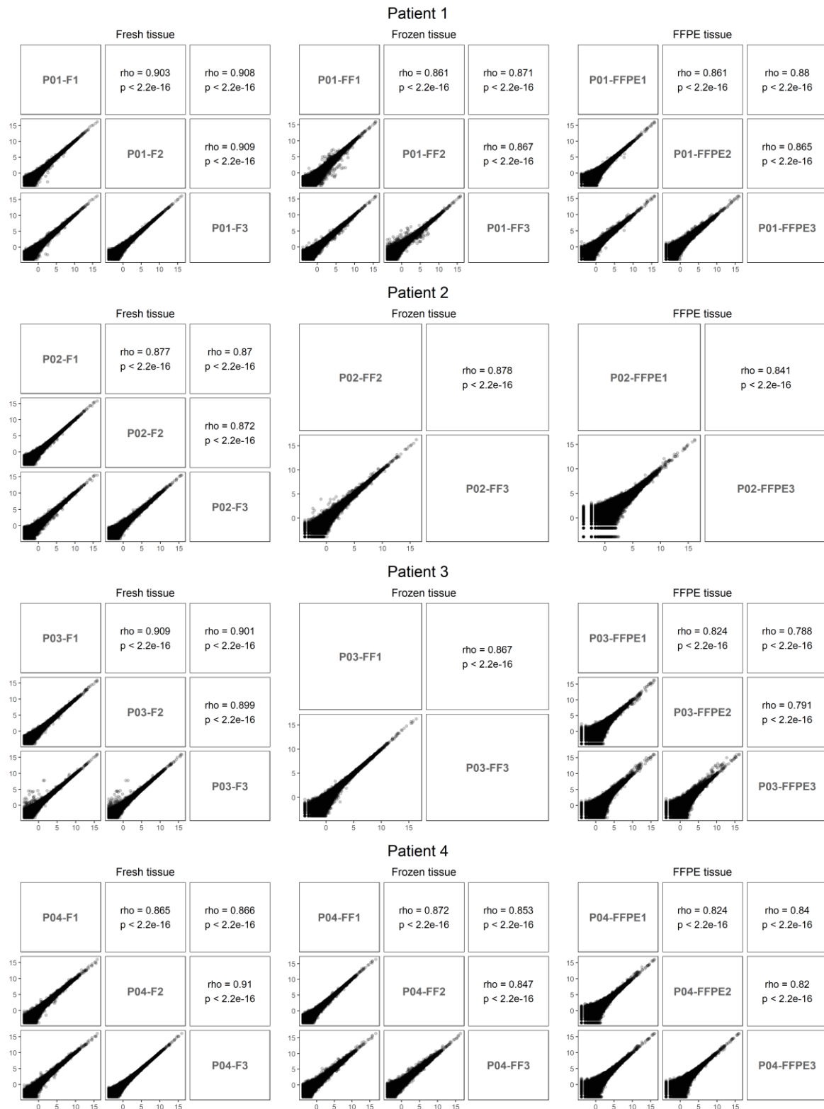
S2 Fig: Spearman's correlation analysis of replicate RNA sequencing investigations in fresh, frozen, and FFPE tissues. Diagonal plots show sample ID, the lower panel shows scatter plots of the paired comparison between gene expression in terms of the \log_2(\text{counts-per-million}) , and the upper panel states the Spearman's correlation coefficient ( \rho ) and p-value ( p ).
