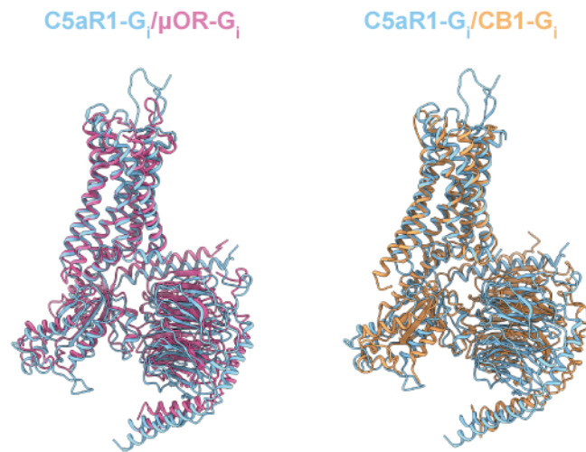
Fig. S4. Structural alignment of C5aR1-G i complex with μOR-G i complex and CB1-G i complex. The superimposition was based on the receptor. Light sky blue, C5aR1-G i complex; hot pink, μOR-G i complex (PDB:6DDE); orange, CB1-G i complex (PDB: 6N4B).
