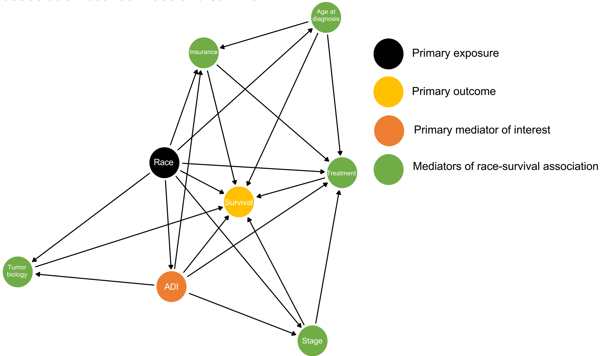
Figure S1. Directed acyclic graph for causal mediation analysis of ADI as a mediator of the association between race and survival
