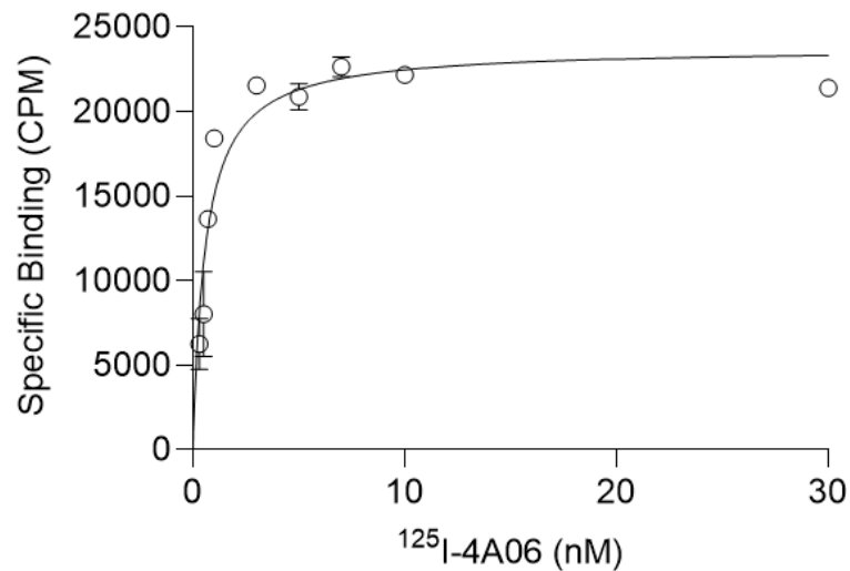
CDCP1 receptor density in UMUC9
