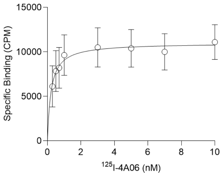
CDCP1 receptor density in 5637
