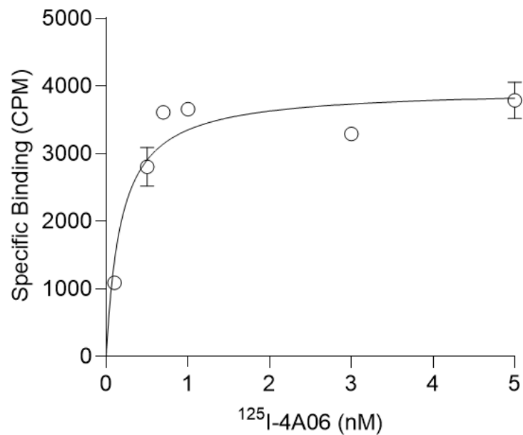
CDCP1 receptor density in UMUC9
