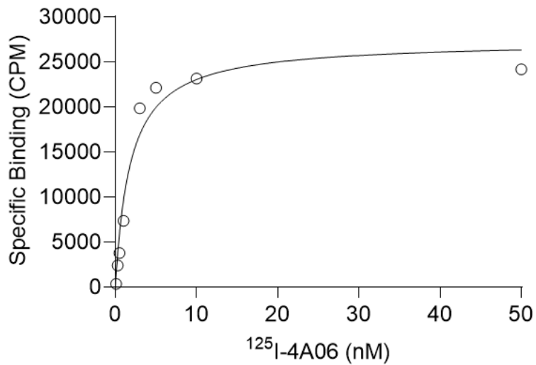
CDCP1 receptor density in UMUC3
