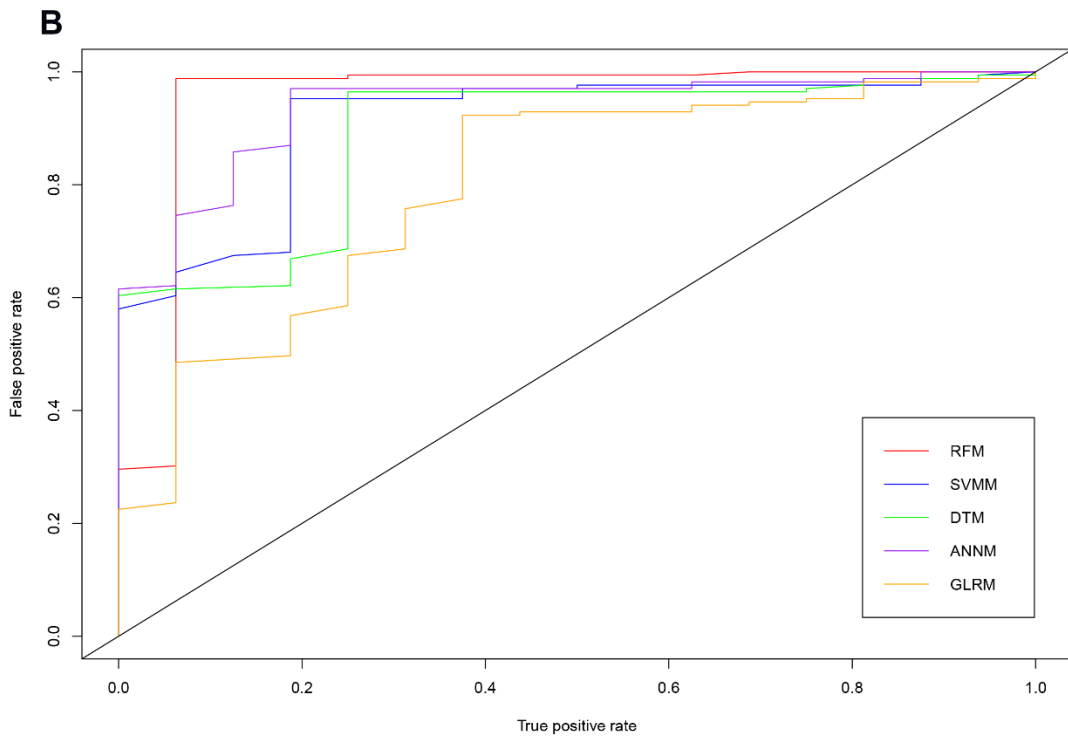
Supplementary Figure 2. ROC curve evaluation of five prediction models.A.Train set;B.Validation set.
