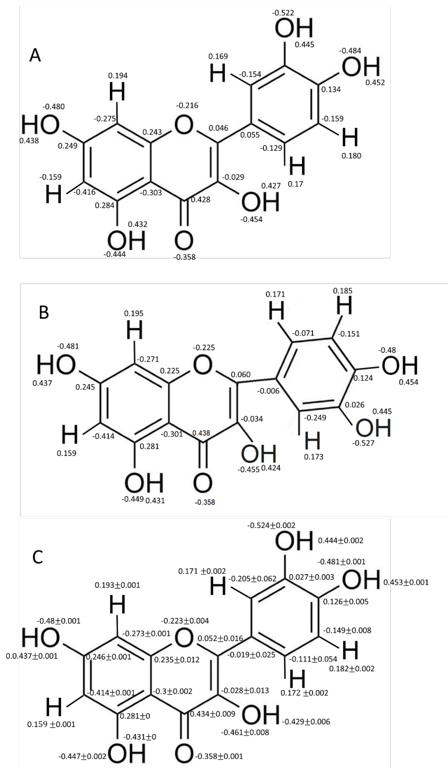
Figure S1. Partial atomic charges of quercetin in configuration A and B. Panel C shows the average value, that was used in the present study.
