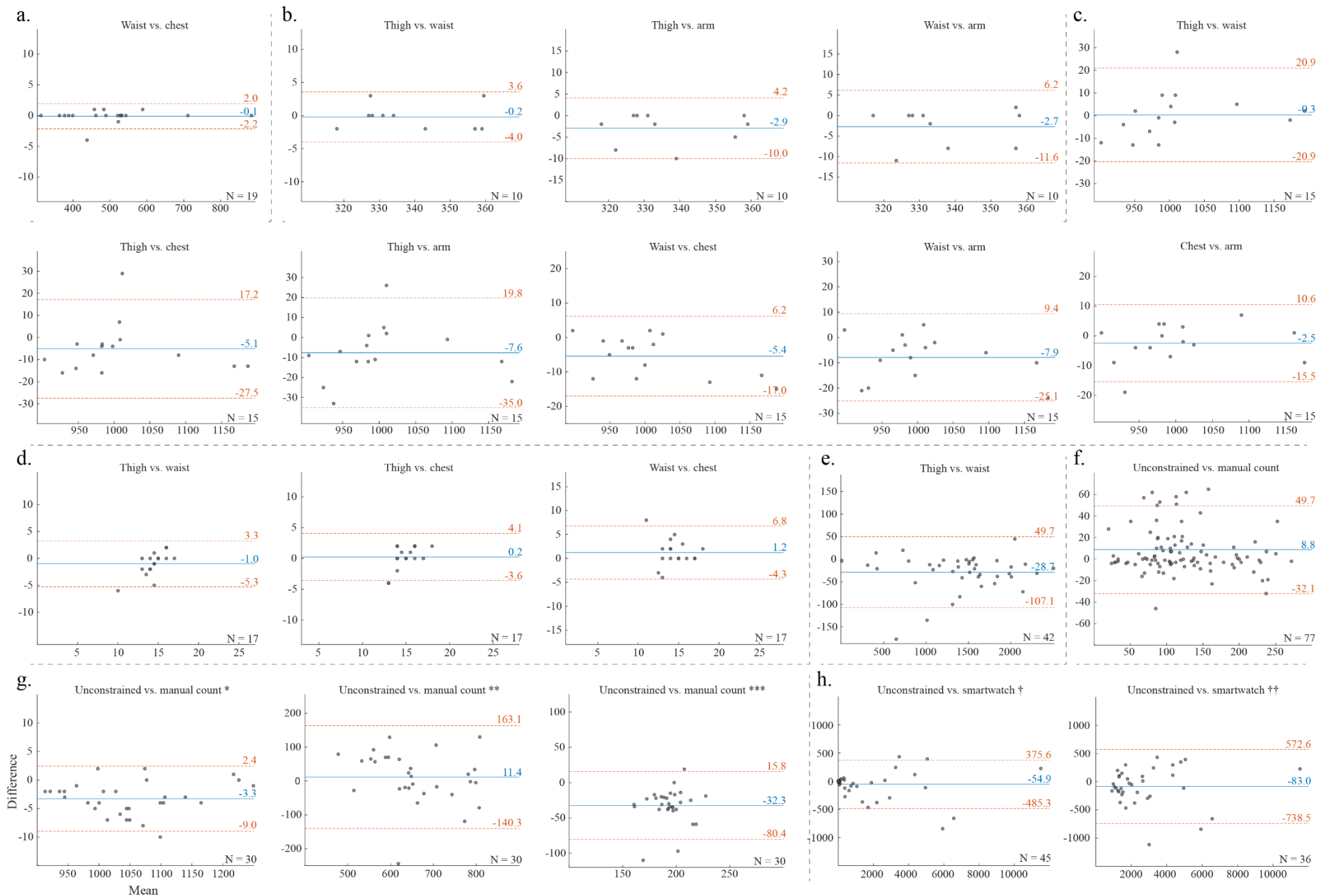
Supplementary Figure 1. Bland-Altman plots with comparison between step estimates in the included studies: DaLiAc (a.), PARUSS (b.), RealWorld (c.), SFDLA (d.), SPADES (e.), WalkRec (f.), PedEval (g.), and HOPE (h.). In PedEval , * indicates task 1, ** indicates task 2, and *** indicates task 3. In HOPE , †
