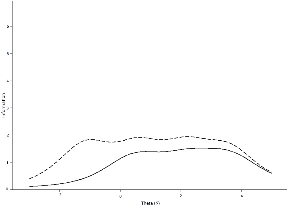
Figure S1. Test information curves for BFI-2 Extraversion (dashed line) and PID-5 Detachment without facet Depressivity (solid line). Note. PID-5 = Personality Inventory for DSM-5; BFI-2 = Big Five Inventory-2; Theta = latent dimension (i.e., personality).
