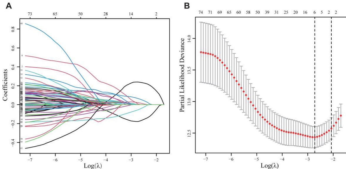
Supplemental Figure 1. Identifying crucial prognosis-related FPTOSs using LASSO regression analysis. (A) Trajectory variation of the independent variable coefficients. (B) The cross validation results of model construction.
