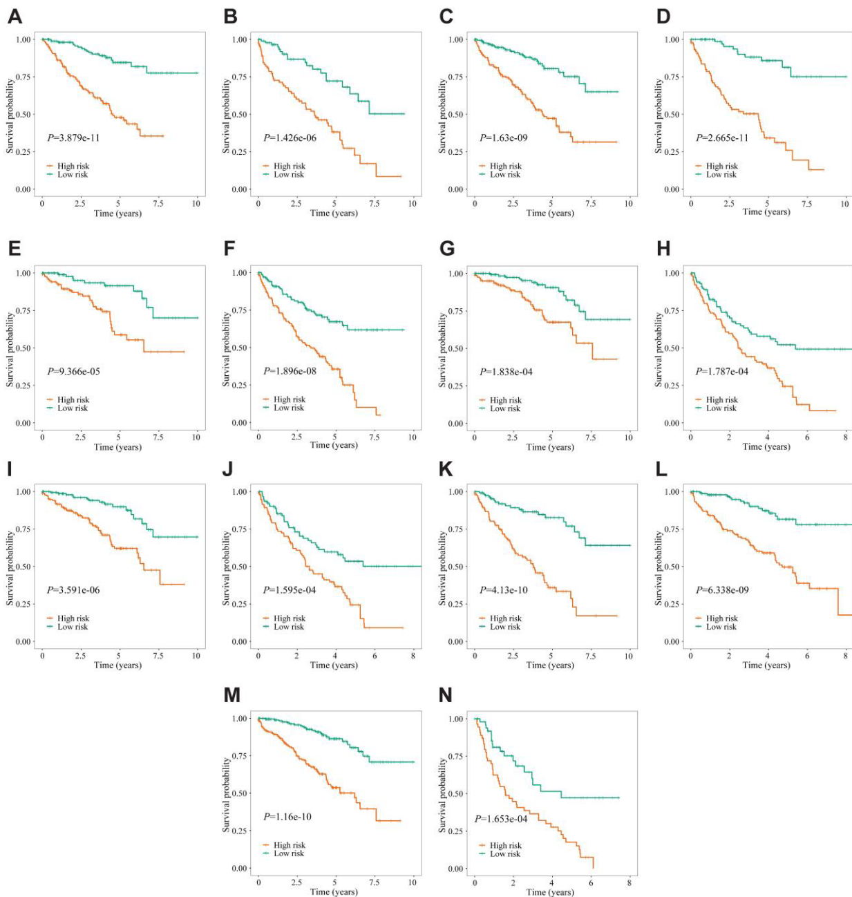
Supplemental Figure 3. Prognostic value of the FPTOS gene signature stratified by various clinical parameters. (A) age \leq 65, (B) age > 65, (C) male, (D) female, (E) grade 1-2, (F) grade 3-4, (G) stage I-II, (H) stage III-IV, (I) T1-2, (J) T3-4, (K) N0, (L) N1-x, (M) M0, (N) M1-x. Log-rank test was applied to compare the statistical differences.
