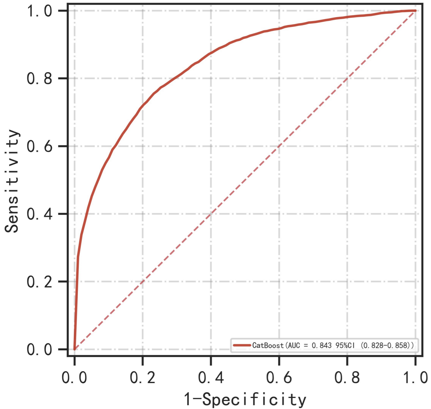
Train ROC Curve
