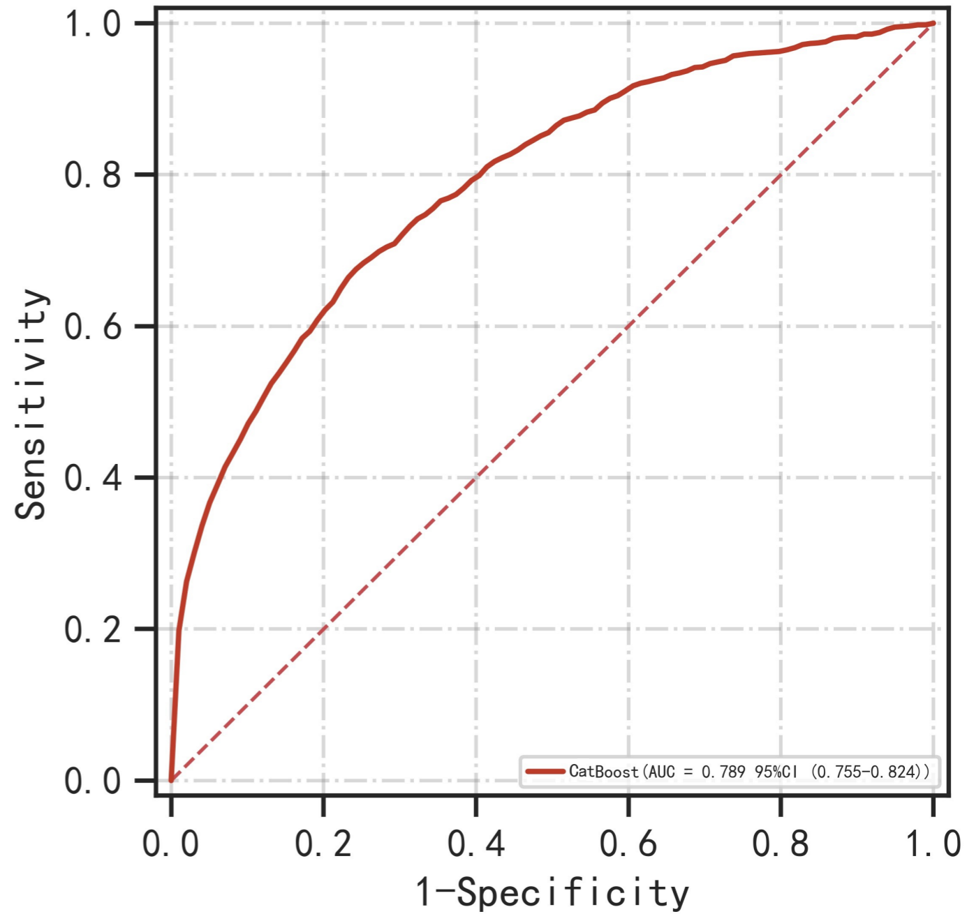
Validation ROC Curve
