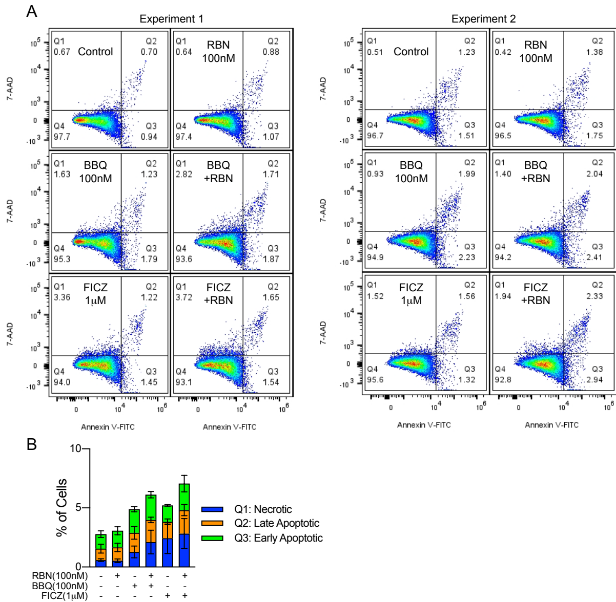
Supplementary Figure 5. FACS analysis of NCI-H660 cells for detection of necrosis and apoptosis.
