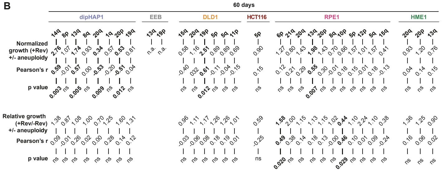
Figure S7. A , Bar graphs representing all arm aneuploidies that are present in >25% of reversine-adapted populations of a given cell type. The grey areas depicts the range (25-80%) in which correlation analysis between copy number changes and fitness was performed for the 90 days time point. Normalized growth with reversine (+Rev) and relative growth (+Rev/-Rev) of the adapted populations with and without the respective aneuploidy as well as corresponding correlation coefficients and p-values are depicted. Growth values were obtained from two independent experiments. B , Correlation analysis as in A , only for the 60 days time point. p-values are from unpaired student's t-test. ns = not significant. n.a. = not assessed.
