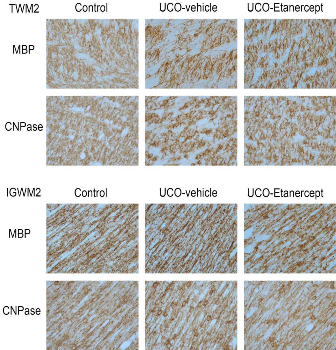
Figure S1: Photomicrographs at 40x magnification of CNPase-positive and MBP-positive labelling in the TWM2 ( Top ) and IGWM2 ( Bottom ) regions. Scale bar = 100 \mu m.
