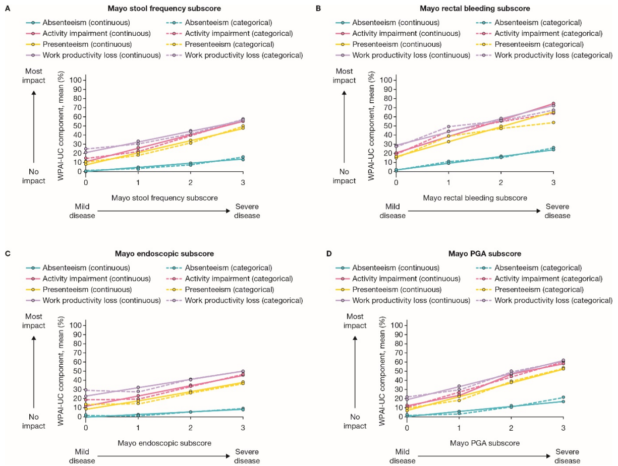
Supplementary Figure 1. Estimated relationship between the Mayo subscores as continuous or categorical anchors and the four WPAI-UC components.
