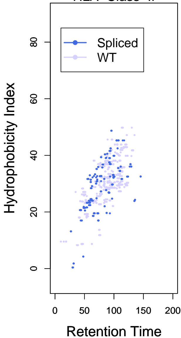
HLA-Class-II
