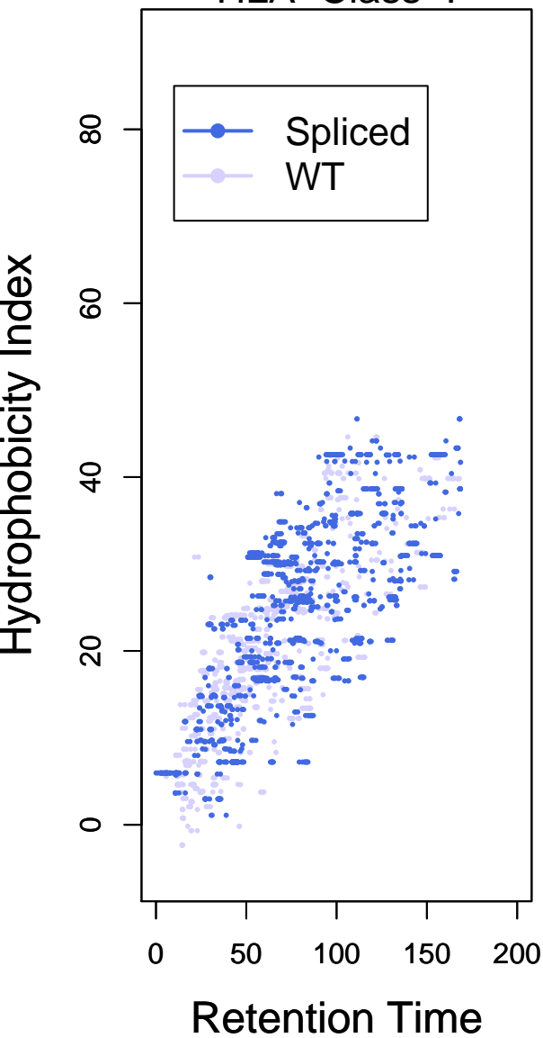
HLA-Class-I
