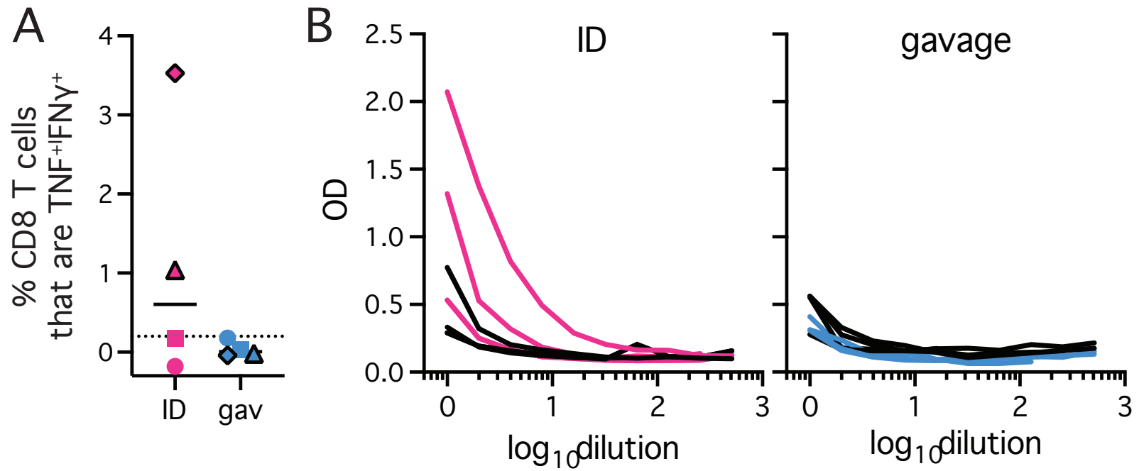
Supplemental Figure 1. Mtb-specific CD8 T cell and IgG responses in the BAL. (A) BAL cells from week 10 post-infection were restimulated with MTB300 and the frequency of IFN \gamma +TNF+ CD8 T cells were measured by intracellular cytokine staining. (B) Mtb-lysate specific IgG responses in the BAL fluid were measured at baseline (black lines) and week 10 (ID: magenta and gavage: blue lines).
