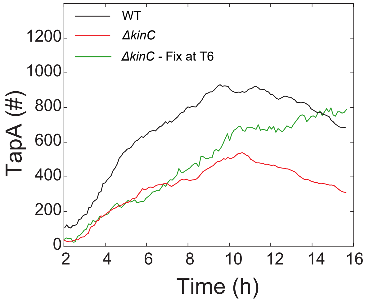
Figure S5: tapA expression is not in a steady-state during simulation. The red and black line shows the dynamics of mean TapA levels of WT and \Delta kinC strains, which are same as Fig. 4B. The green line shows the mean TapA levels of \Delta kinC strain supposing the growth rate stops to decrease and fixed at T6.
