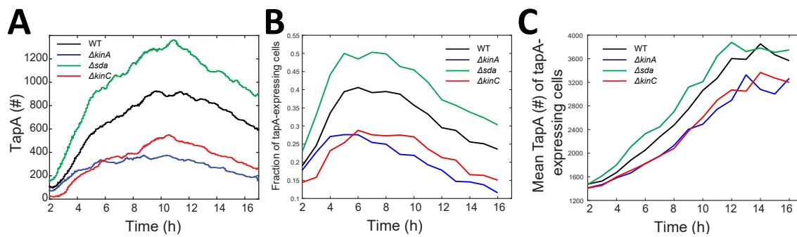
Figure S7: Effects of tapA-expressing cell fraction and tapA-expressing levels.
