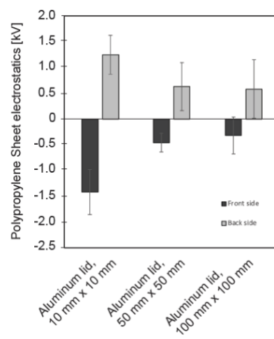
Figure S2: Aluminum lid size dependence on the polypropylene sheet charging capability.
