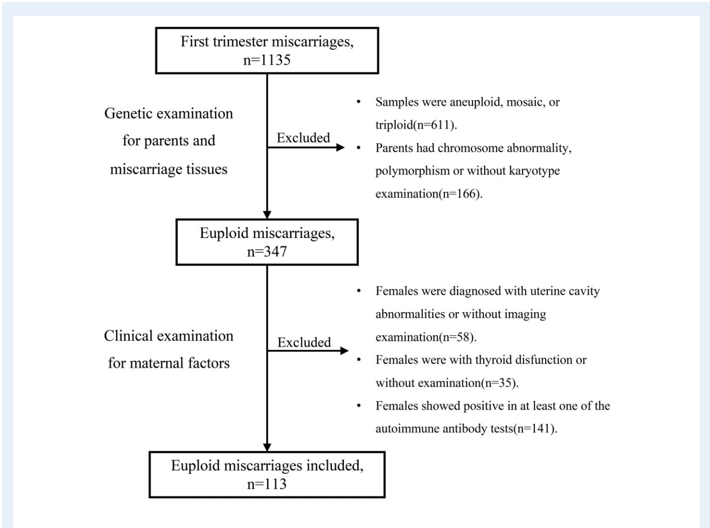
Supplementary Figure S6. Flowchart of euploid miscarriages included in multiplex PCR for RYR2 and PLXNB2 sequence.
