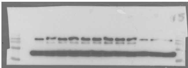
FoxO3a/Actin
