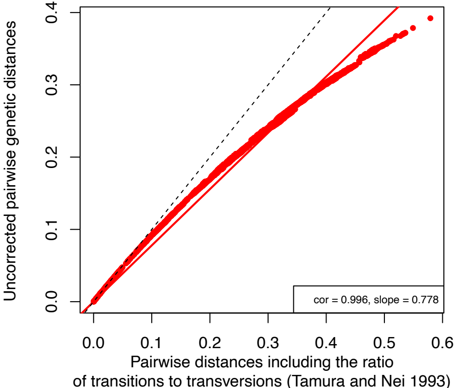
Suppl. Figure 1. Substitution saturation plots for A) Hexacorallia and B) Octocoralla.
