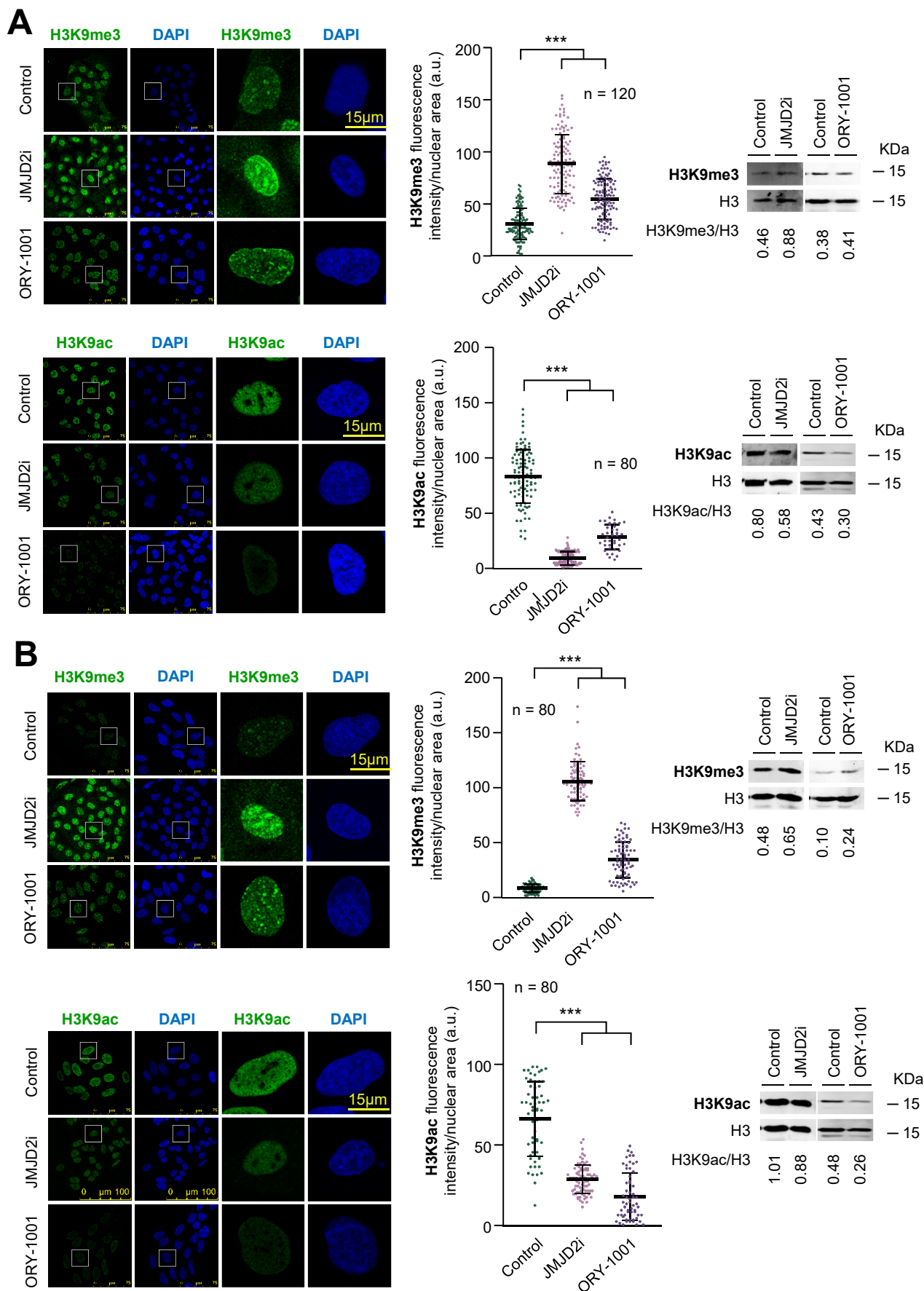
Figure S12. Effect of KDM inhibitors on H3K9 acetylation and methylation in A549 (A) and U2OS (B) cells. The quantification of the fluorescence is shown in the middle. The immunoblots are shown on the right.
