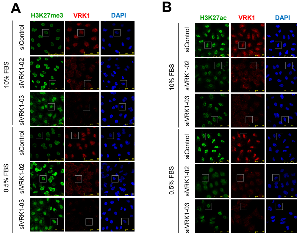
Figure S3. Effect of VRK1 depletion on the epigenetic modifications of H3K27 in the presence (top) or absence (bottom) of serum in A549 lung adenocarcinoma cells. A. Effect on H3K27me3. B. Effect on H3K27ac. The boxes indicate the selected cells shown in Figure 2. The selected cells are indicated by a square. siCt: siControl; siV-02: siVRK1-02; siV-03: siVRK1-03.
