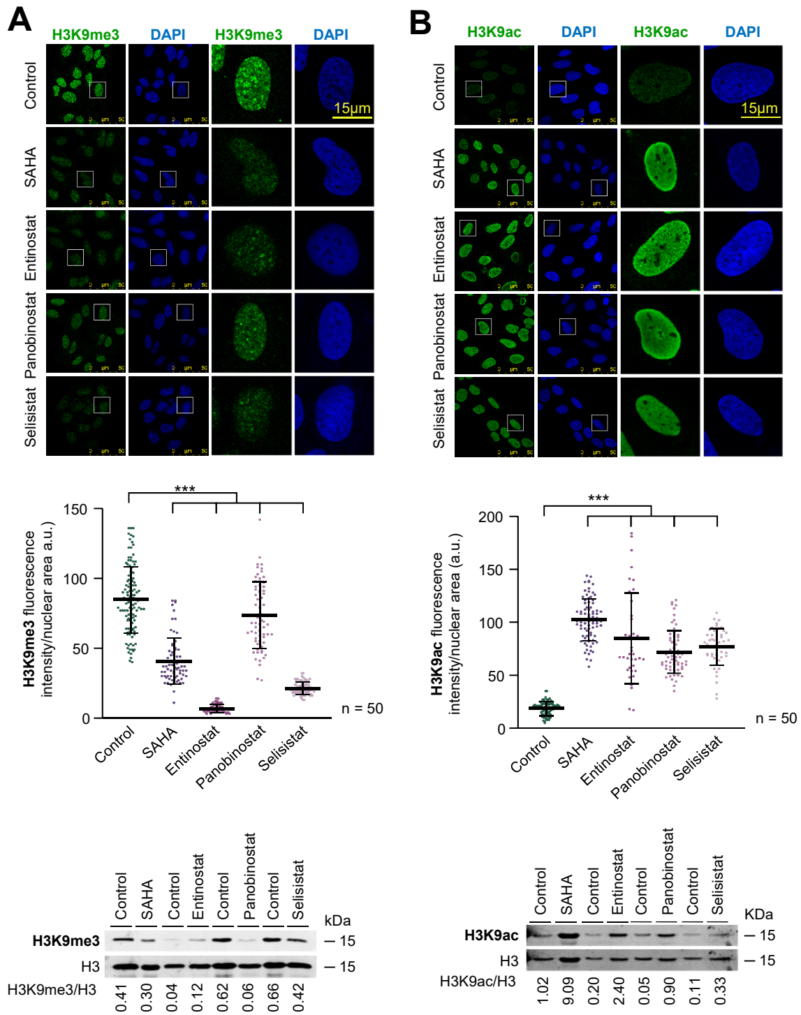
Figure S9. Effect of HDAC inhibitors on histone H3K9 epigenetic modifications in serum-deprived U2OS cells. A. Effect of HDAC inhibitors on H3K9me3 levels. B. Effect of HDAC inhibitors on H3K9ac levels.
