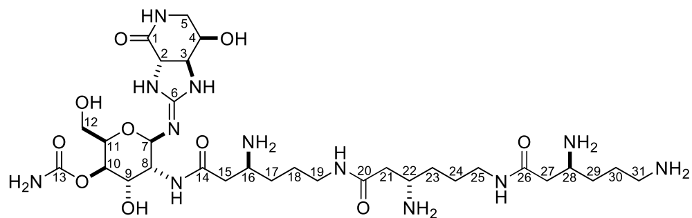
Streptothricin D
