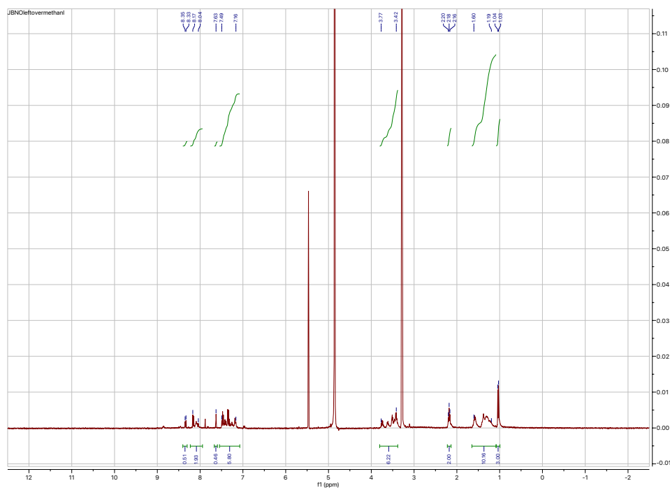
Figure MS 1B. ^1\text{H} NMR of Nitroso-DTB.
