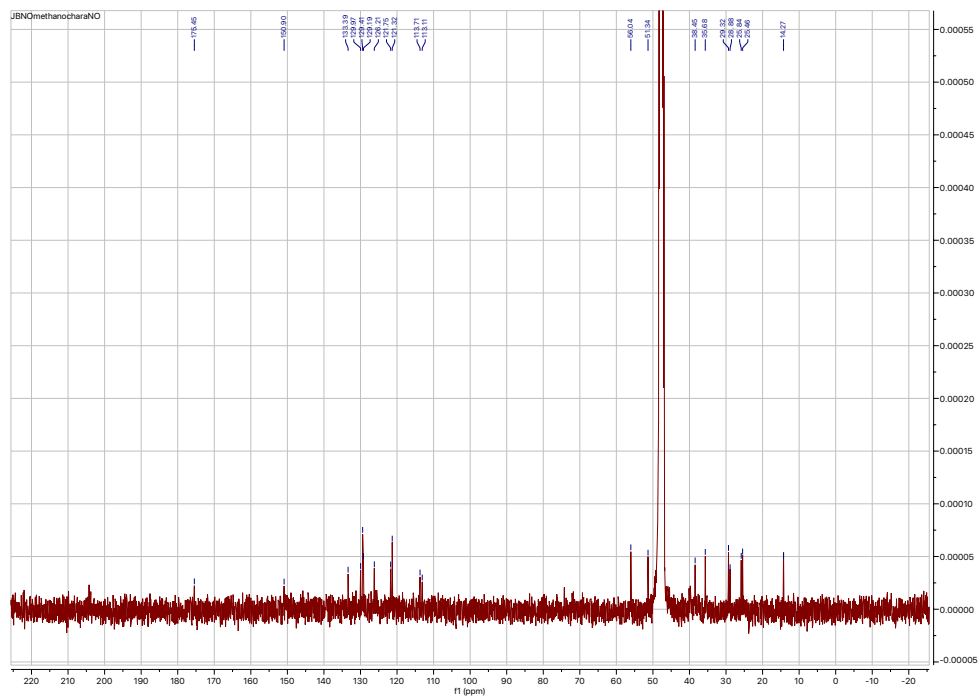
Figure MS 1C. ^{13}\text{C} NMR of Nitroso-DTB.
