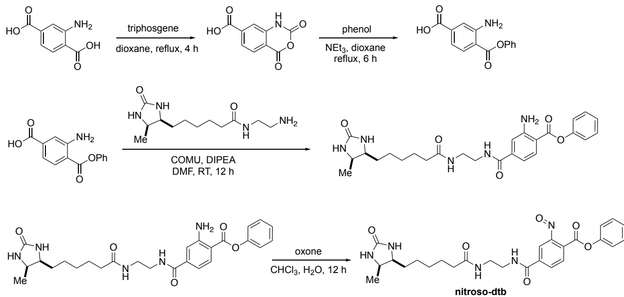
Figure MS 1A. Synthesis of Nitroso-DTB.
