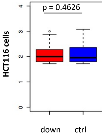
A. Positive strand
