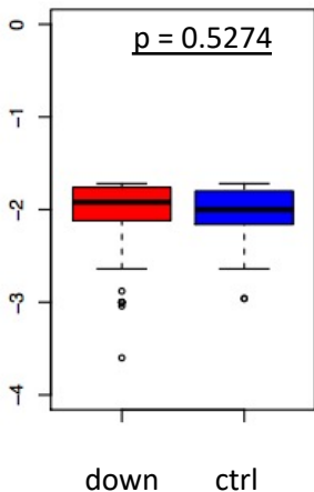
B. Negative strand
