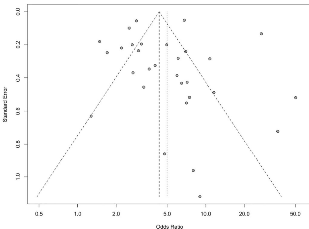
Supplementary Figure S4. Funnel plot of obesity meta-analysis. X-axis = non-linear scale. Thin dotted line = mean odds ratio. Egger regression test of funnel plot asymmetry. Test result: t = 0.31 , df = 28 , P\text{-value} = 0.7558 .
