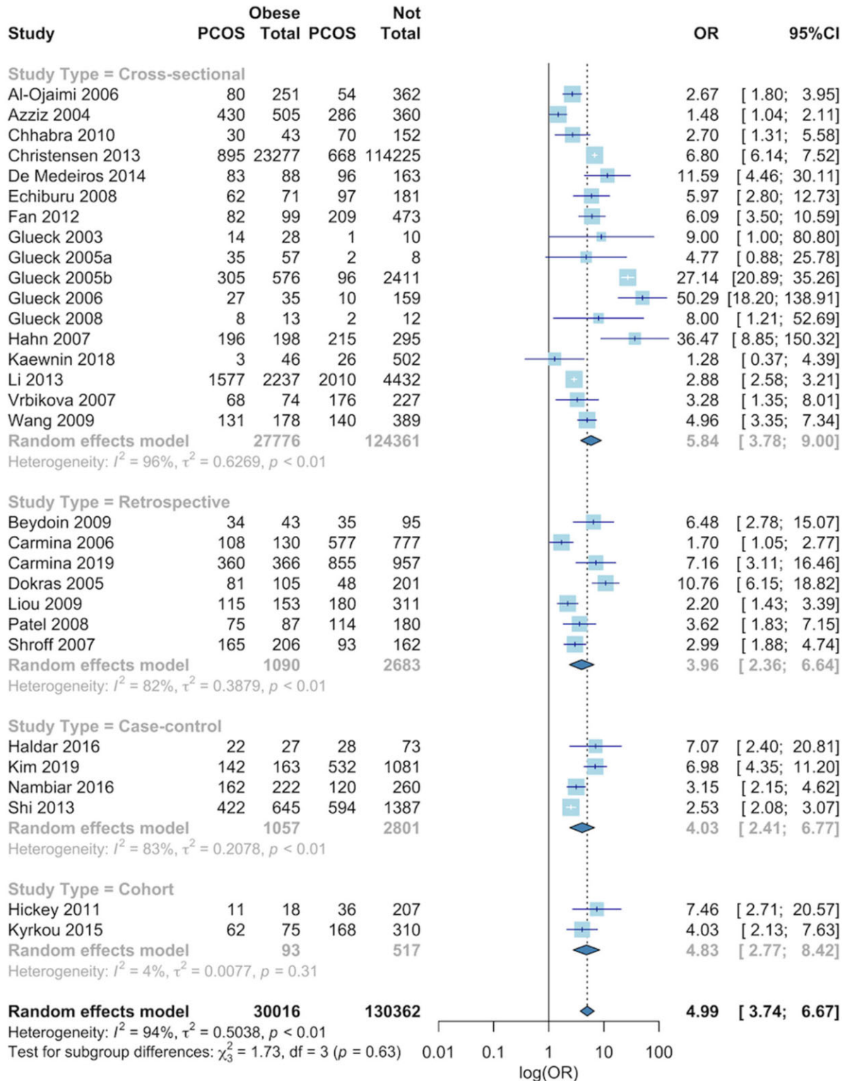
Supplementary Figure S7. Obesity meta-analysis by study type. Forest plot for odds ratio of PCOS in obese vs non-obese. OR: odds ratio.
