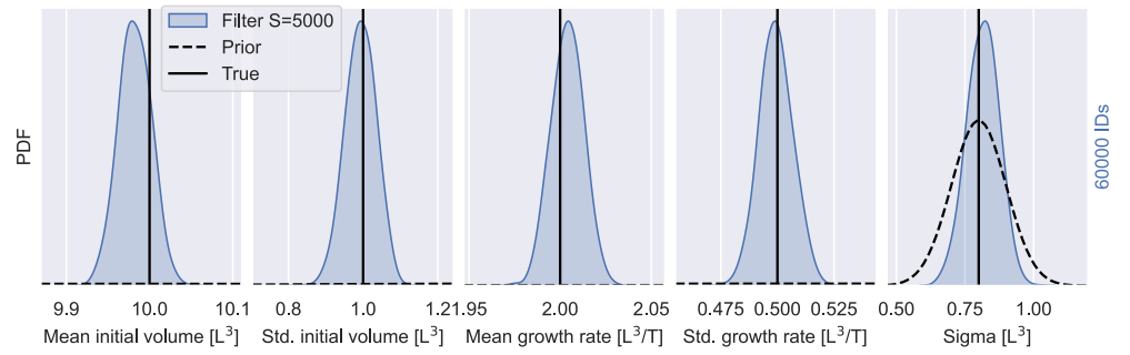
S3 Fig. IIV-noise identifiability of early cancer growth model II. The figure is an extension of S1 Fig and shows filter inference results for the early cancer growth model from 60 000 snapshot measurements using Gaussian filters with S = 5\,000 simulated individuals. The prior distributions are illustrated by black dashed lines and the data-generating parameter values are depicted by solid black lines.
