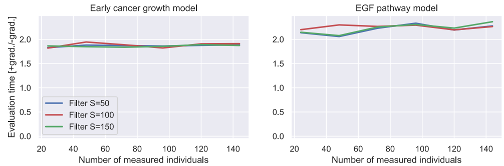
S4 Fig. Computational costs of log-posterior evaluation with and without gradients. The figure is an extension of Fig 7 and shows the evaluation time of the filter log-posterior with gradients in units of the evaluation time of the filter log-posterior without gradients for different numbers of measured individuals. The evaluation times are estimated according to S7 Text. The left panel shows the results for the early cancer growth model and the right panel the results for the EGF pathway model for S = 50 (blue), S = 100 (red) and S = 150 (green) simulated individuals.
