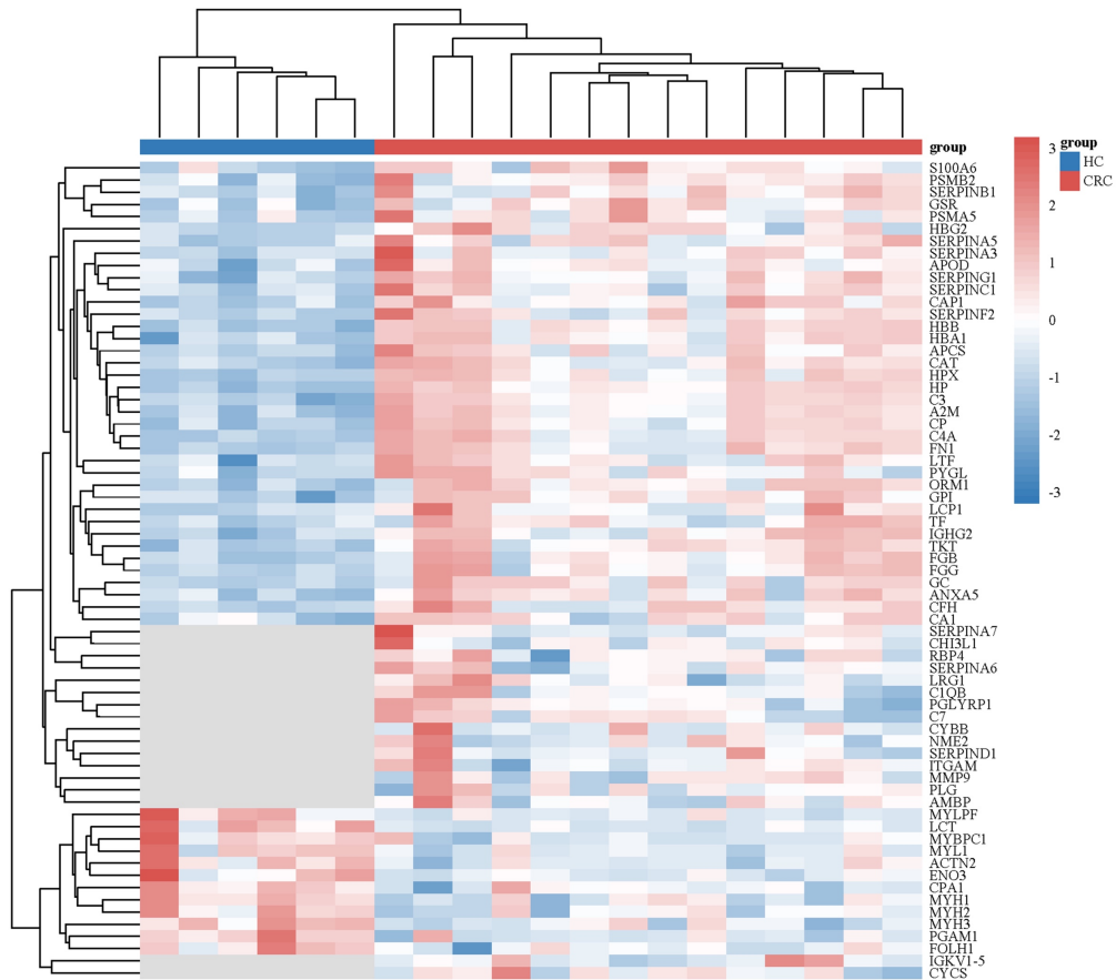
Supplementary Figure 3. Cluster heatmap of 67 differentially expressed stool proteins according to more stringent criteria. The criteria for differential expression of proteins were |\log_2\text{-fold change}| > 1 and P < 0.01 .
