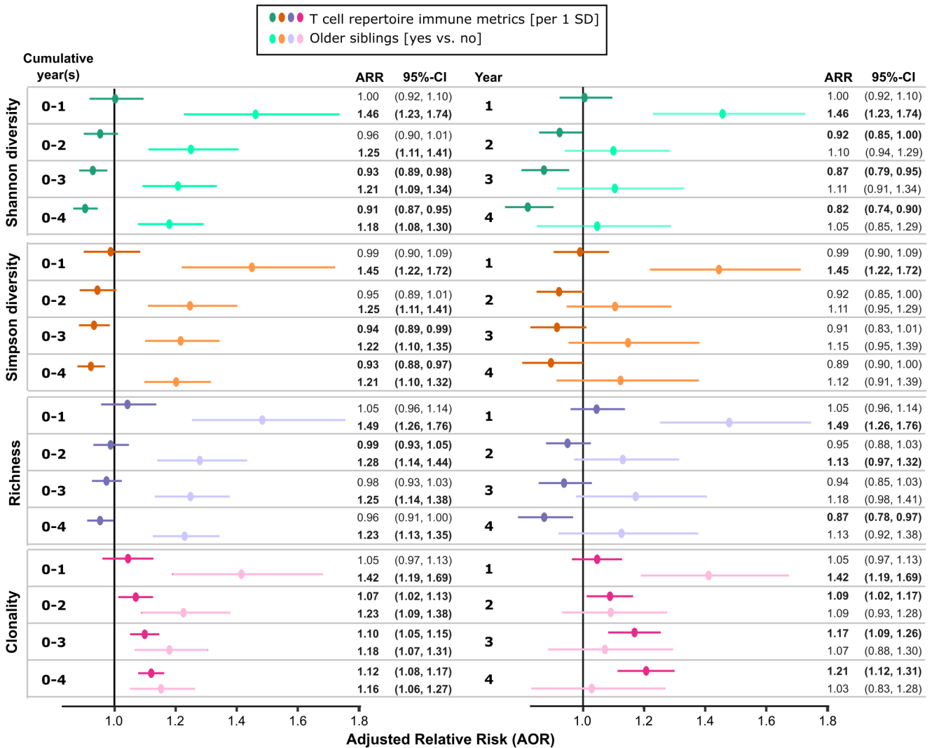
Supplemental Figure 3: Poisson regression analysis of the cumulative number of ARI at the age of 1, 2, 3, and 4 years and in the respective years alone. Separate models show the association for each T cell repertoire immune metric (Shannon diversity, Simpson diversity, richness, clonality) in comparison with the effect of having older siblings, while mutually adjusting within each time frame or year (n=67). Estimates and 95% confidence intervals are shown.
