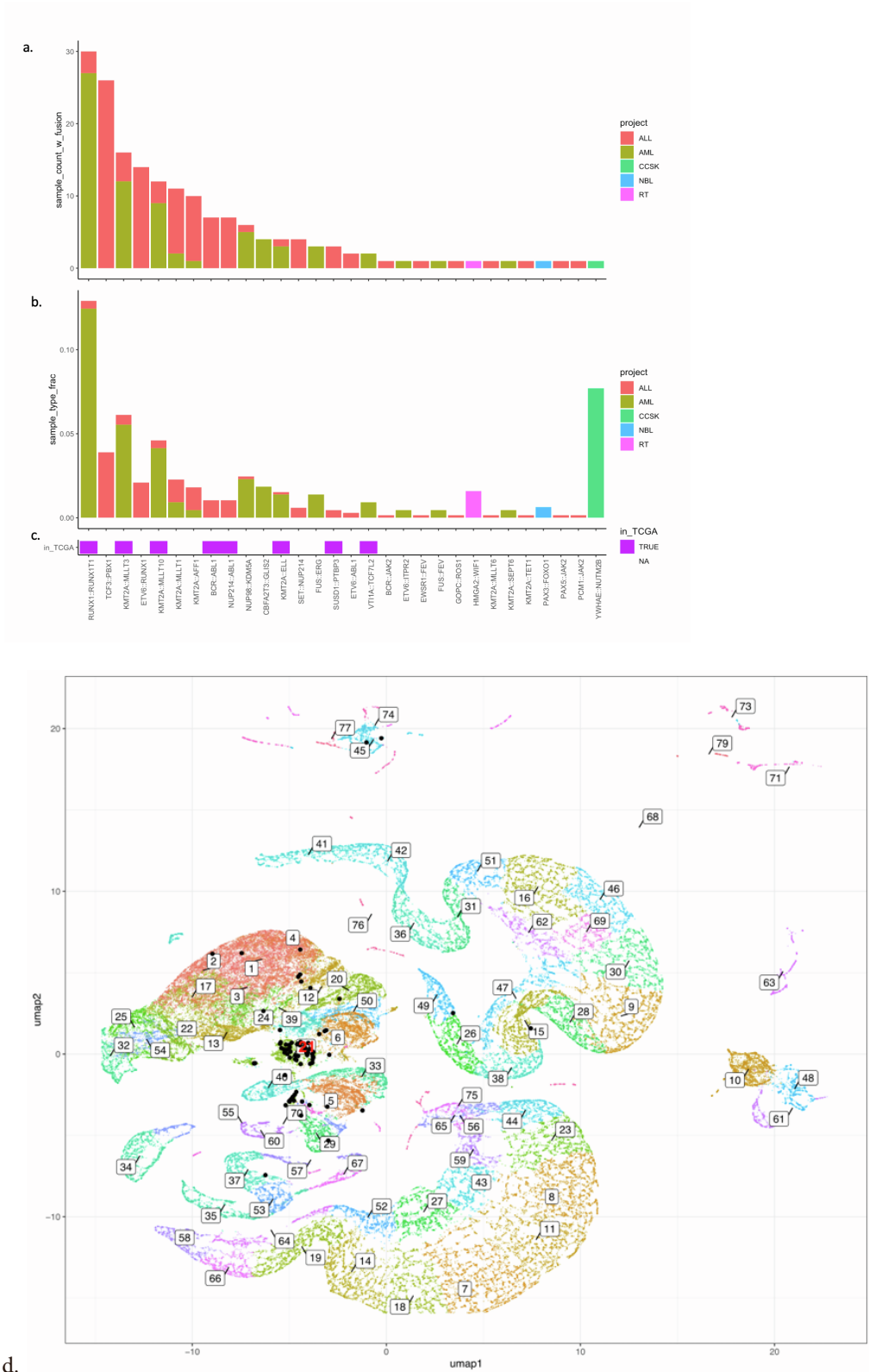
Figure S9: FusionInspector Exploration of TARGET Pediatric Cancers. (a-c) 30 COSMIC Fusions Found in Samples Among TARGET Pediatric Cancers. (a) Counts and (b) fractions of project participants containing corresponding COSMIC fusion. (c) Indicator shown for COSMIC fusions found among TCGA samples. Note that
