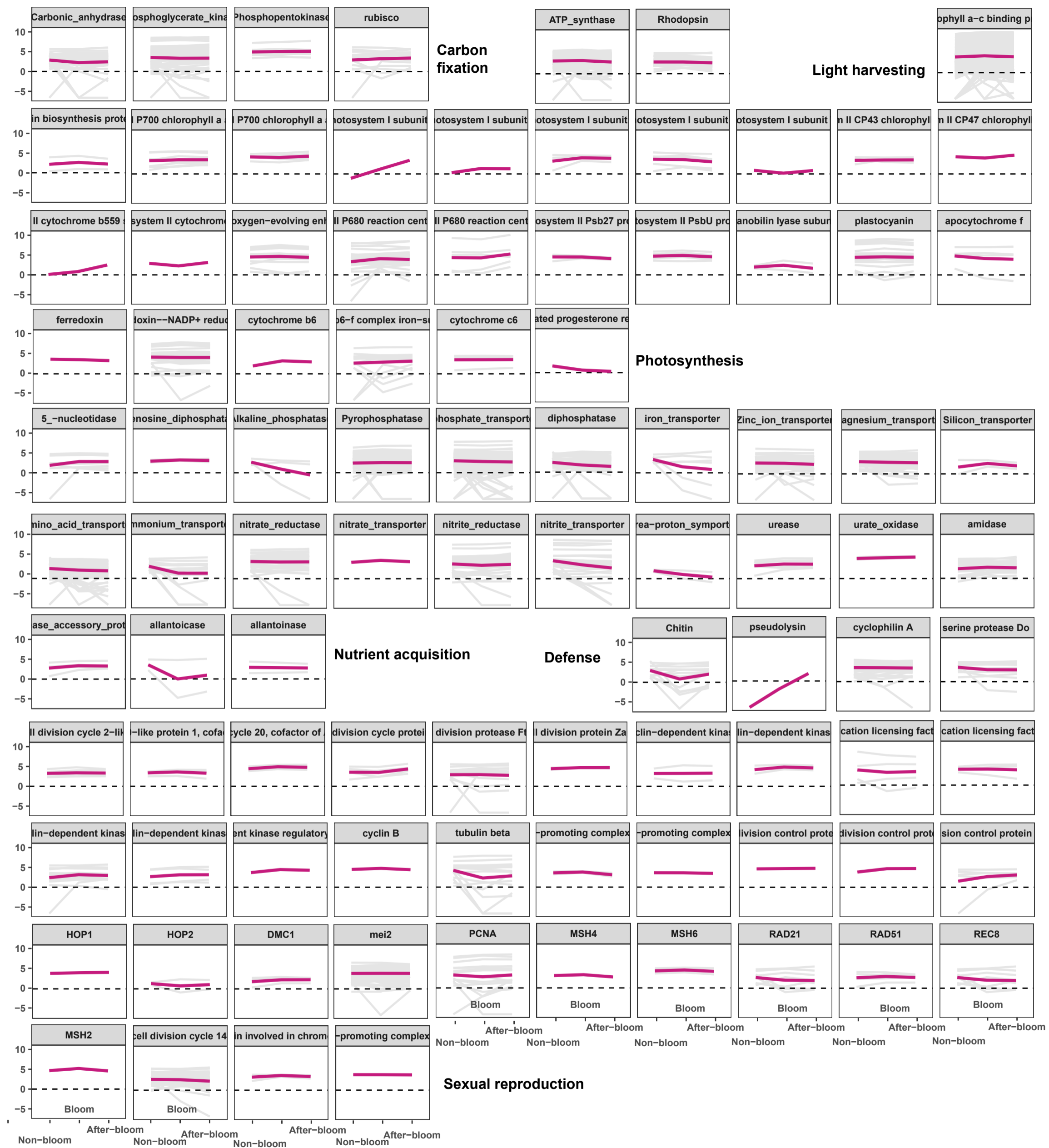
Fig. S1. Expression patterns of energy and nutrient acquisition, defense, and cell reproduction (ENDS) related genes in Karenia under the three bloom conditions (non-bloom, bloom and after-bloom).
