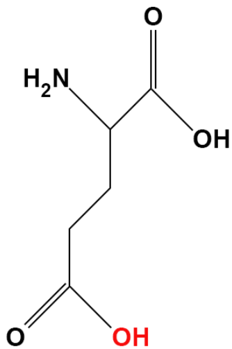
Glutamic Acid
