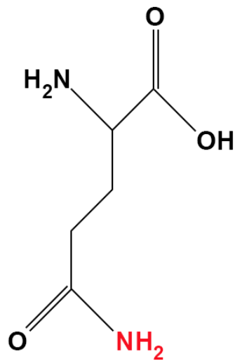
Glutamine
