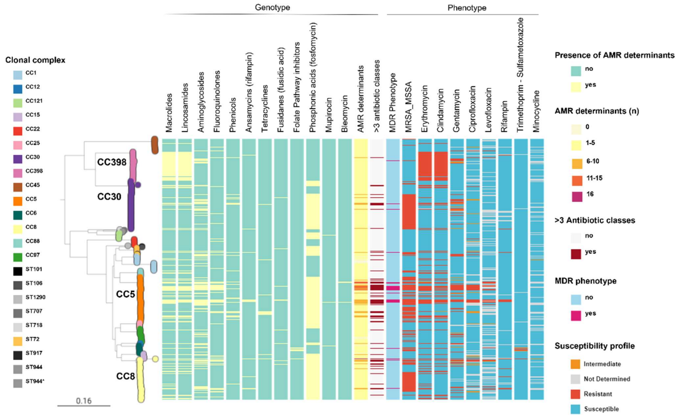
Supplementary Figure 4. AMR determinants and AMR phenotypes. Maximum Likelihood tree of 404 genomes inferred from 156868 SNP sites identified on 2182 core genes (Panaroo) with RAxML. Midpoint rooted. 500 bootstrap replicates. Tree nodes and blocks are coloured as described in the legend.
