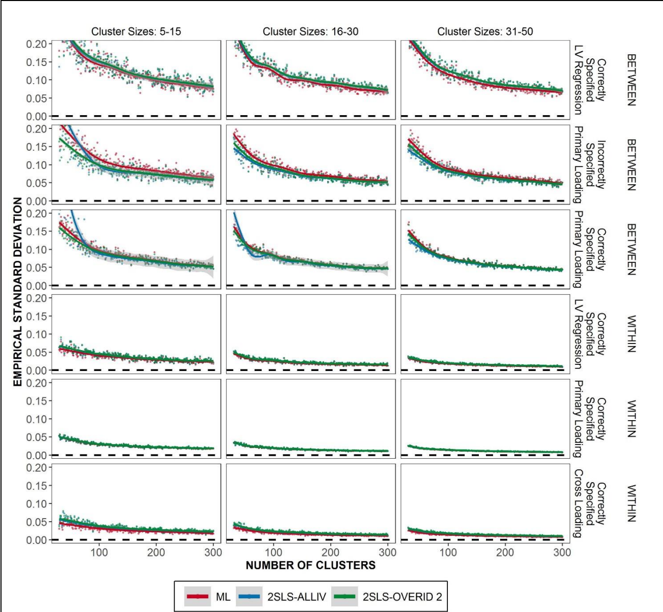
Figure 14. Empirical standard deviations of parameter estimates given the Misspecified Between Model .
