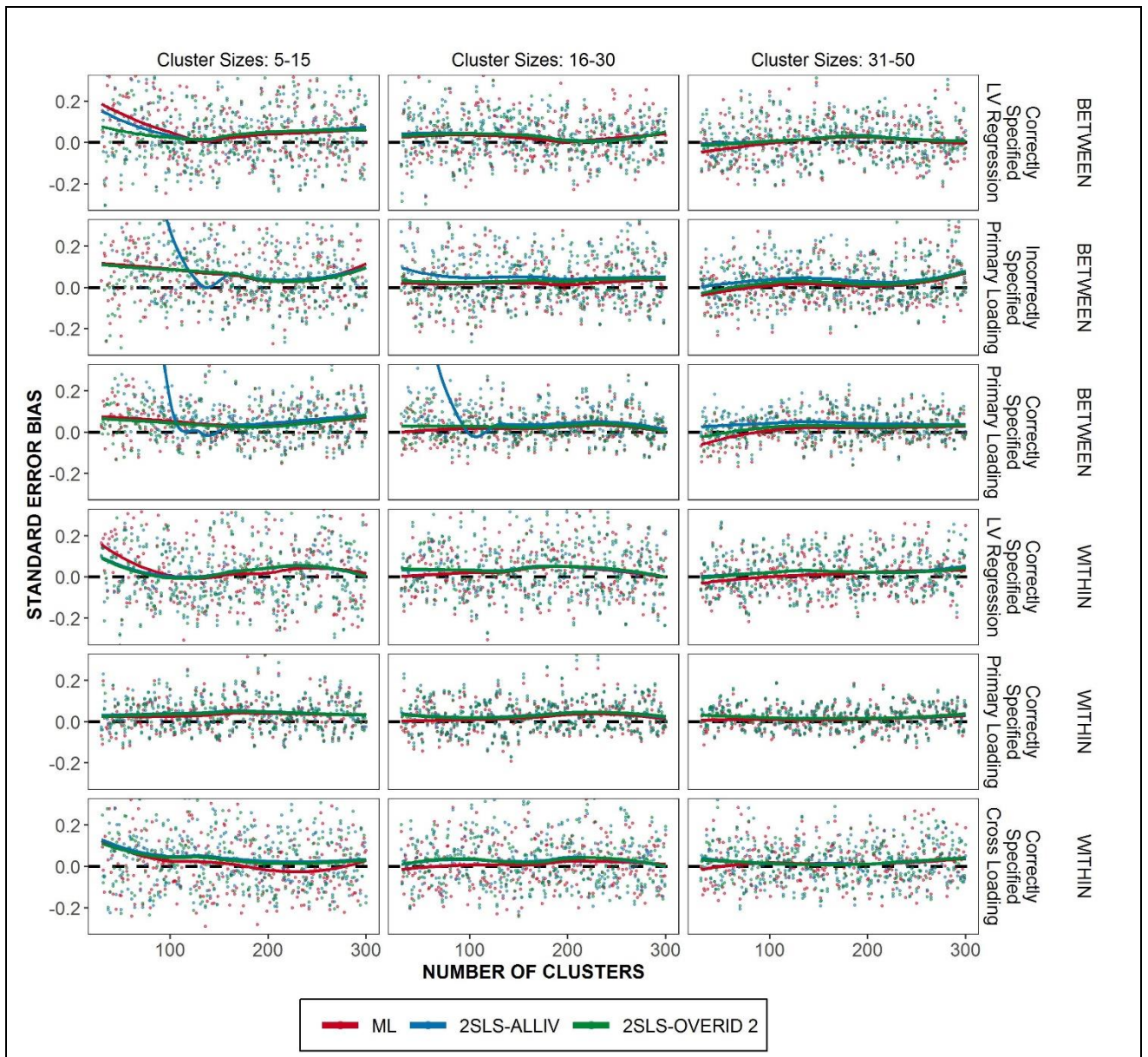
Figure 16. Standard Error Bias given the Misspecified Between model.
