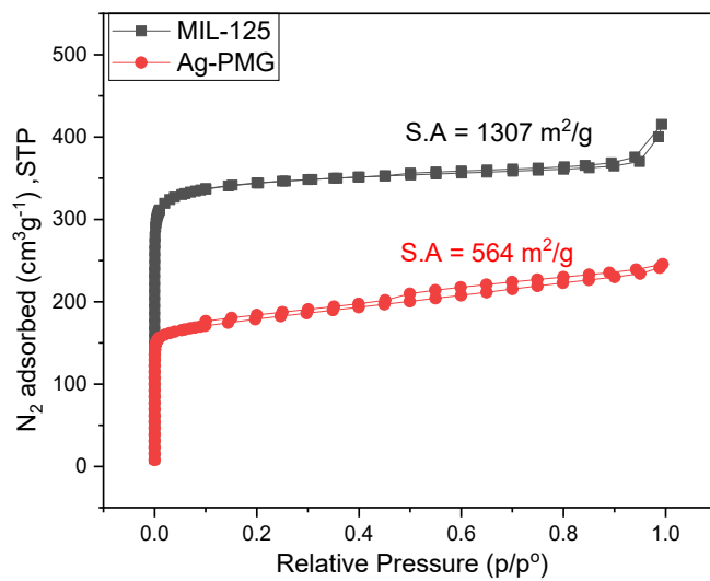
Fig. 2S. N 2 adsorption-desorption isotherms for MIL-125 and Ag-PMG
