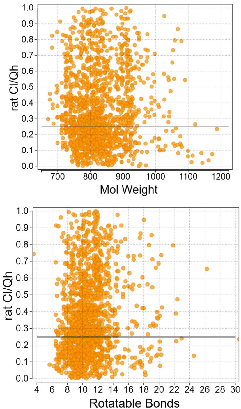
Figure S2. Clearance in rats as a function of physicochemical descriptors.
