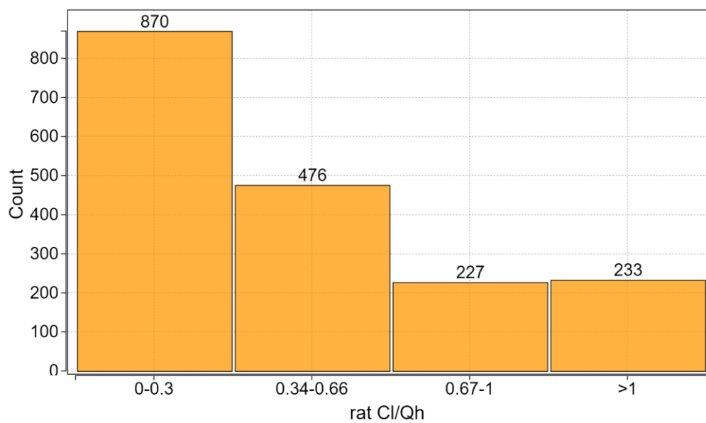
Figure S1. Cl/Q_h in rats for the compounds in the dataset.
