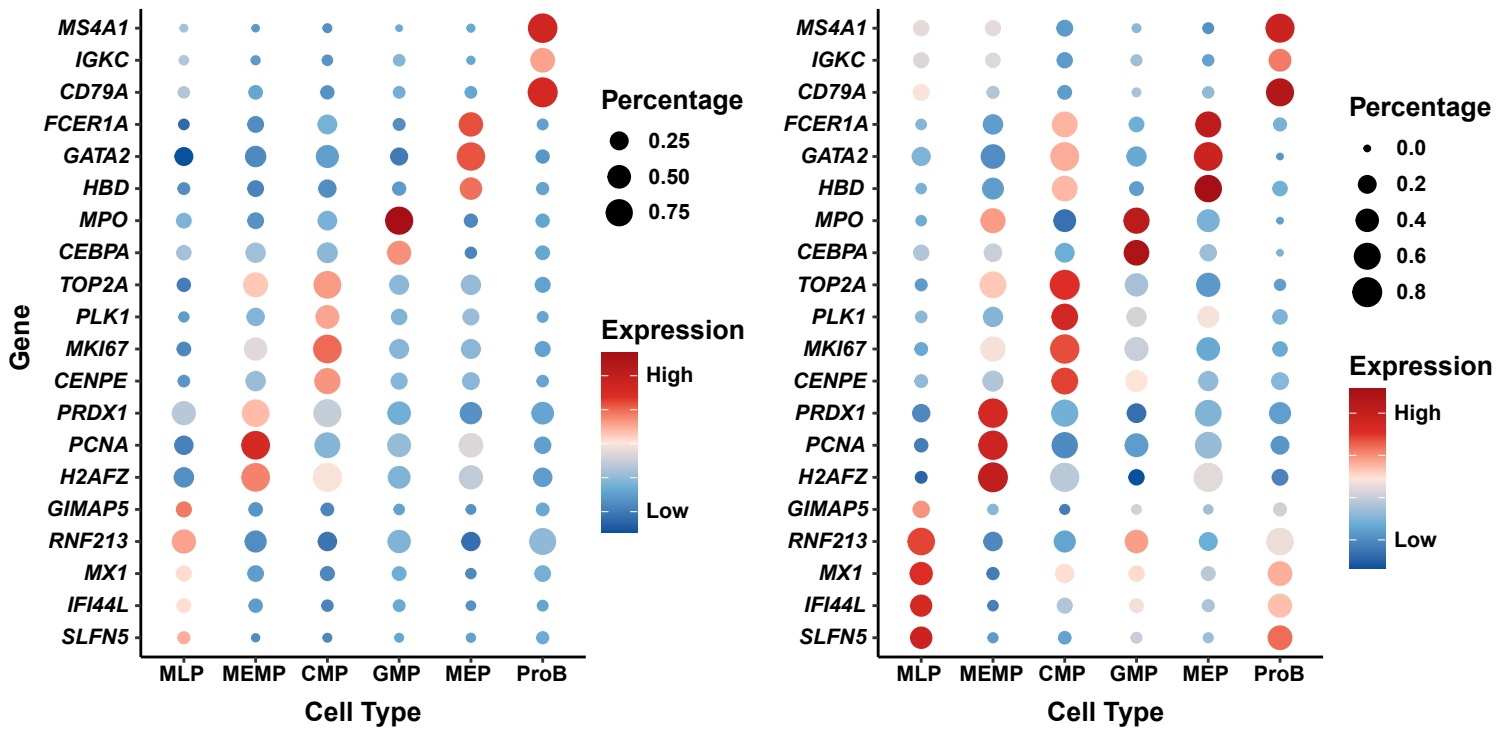
Figure S1. Samples information and the expression of cell type-specific genes in reference and query data.
