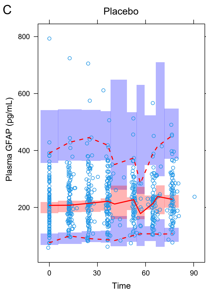
Supplemental Figure 1. Visual predictive check of final plasma biomarker models.
