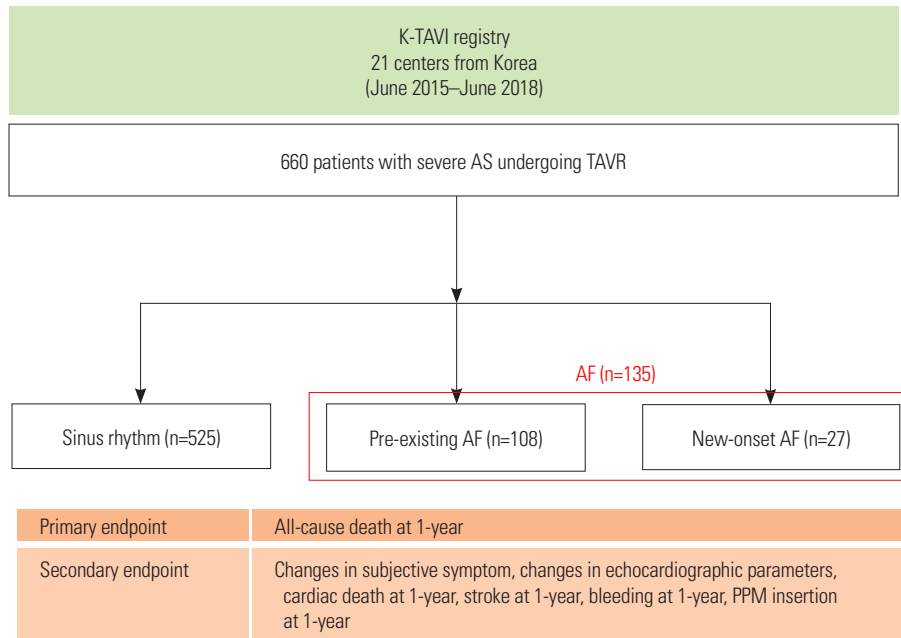
Supplementary Fig. 1. Study flow. A flow diagram is shown. AF, atrial fibrillation; AS, aortic stenosis; PPM, permanent pacemaker; TAVI, transcatheter aortic valve implantation.
