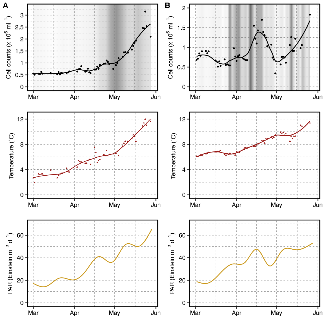
Figure S1 Total DAPI-stained cell counts with chlorophyll a concentration (grey, background), temperature, and photosynthetically active radiation (PAR) during the spring phytoplankton bloom (A) 2018 and (B) 2020.
